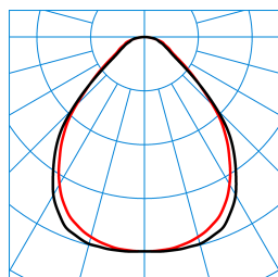
ArmoFit M73 PW19 52-830 ETDD + ArmoFit Sky M73-TS ZER TX426943
