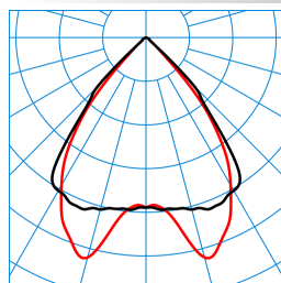
SFlow D2-L MRX LED4000-830 ET 01 TX723887
