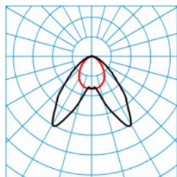
ELINE LDAW40-110 ML 840 L150 2 20
