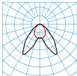
ELINE LDAW40-110 ML 840 L150 4 20
