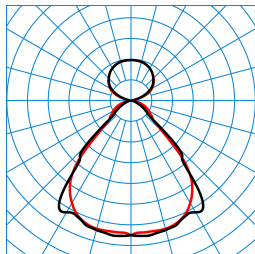
SFlow-Act H2-L MRW LED6400 ETDD8 03 (ActDCW) TX299746
