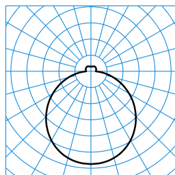
Solegra D3 OTA 13500-840 + ZS A 5075/3000 TX772940
