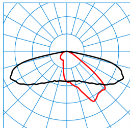
LIQ 50N-AB2L-LR/4600-730 6G1 ET (CLO end value) TX777908
