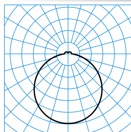
Olisq RWD3 DW 30-840 ETBLE +CAS-S TX565800
