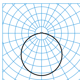
Olisq RWD3 DW 30-840 ETBLE +CAS-S + Olisq RWD3 C 01 TX565801
