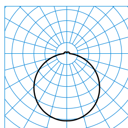
Olisq Act RWD4 DW 40 ETDD8 PC (ActDCW) TX375938 ■ C0 - C180 ■ C90 - C270
