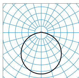
Olisq Act RWD4 DW 40 ETDD8 PC + Olisq RWD4 C 01 (ActDWW) TX426998 ■ C0 - C180 ■ C90 - C270
