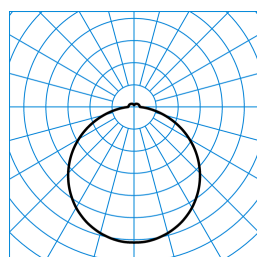
Olisq Act RWD4 DW 40 ETDD8 PC (ActDSU) TX376237 ■ C0 - C180 ■ C90 - C270
