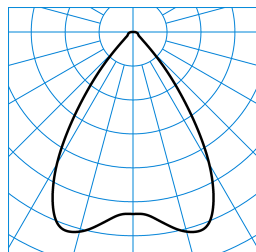
InperiaL G2 C07 BR19 1800-830 03 + ZN-PC ■ C0 - C180 TX052827
