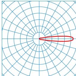
CS 19 S-MOD RE6R/2200-740 1G1 ETDD (CLO end value) TX369163
