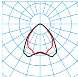
ELINE HE LW60-160 ML 830 L225 0 20 ■ C0 - C180
