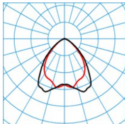
ELINE HE LW60-160 ML 830 L225 2 20
