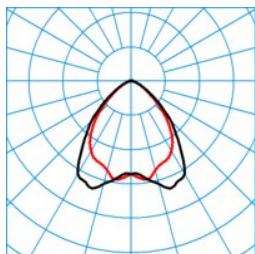
ELINE HE LW60-160 ML 830 L225 4 20 ■ C0 - C180
