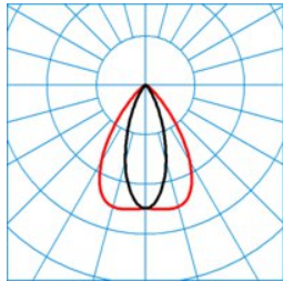
ELINE HE LVN40-120 ML 865 L150 0 20 ■ C0 - C180
