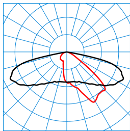
LIQ 50N-AB2L-LR/350/420/460-722 6G1 ET (CLO initial value) TX776342
