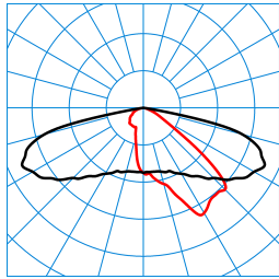
LIQ 50N-AB2L-LR/350/420/460-722 6G1 ET (CLO end value) TX776340
