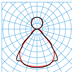
SFlow H3-L MRW LED6400-840 ETDD LLWS 03 TX719552
