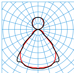
SFlow H3-L MRW LED6400-840 ETDD LLWS 03 TX721313
