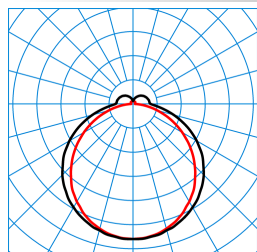
Olisq Act LWD3 DW 30 ETDD8 IP54 IK (ACTDWW) TX430080
