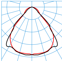
SFlow C3-L MRW LED4000-840 ETDD LLWS 01 TX771985
