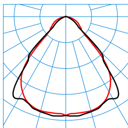
SFlow C3-L MRW LED4000-840 ETDD LLWS 01 TX721319
