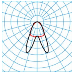
ELINE LDAN40-110 ML 830 L150 4 50 ■ C0 - C180 DIN 5040 = A50 UGR I 3 = 24,3 UGR q 3 = 25,0 UTE 3 = 0.99 C + 0.01 T CEN flux code = 64 88 97 99 100 0 7 47 1
