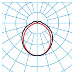
ELINE DL35-100 ML 830 L150 4 20
