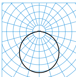
Olisq RWD2 DW 20-830 ETBLE +CAS-S IP54 + Olisq RWD2 C 01 TX565945
