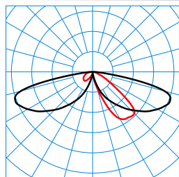
LTX LT-AB2L-LRA/15/18/26-740 4G1 (1500 lm) TX084097
