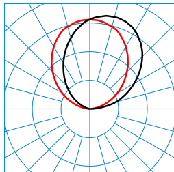
SanescaAct W2 5000 ETDD8/ET 840 03 ACTDWW (room light) TX301990
