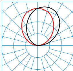
SanescaAct W2 5000 ETDD8/ET 840 03 ACTDCW (room light) TX302000
