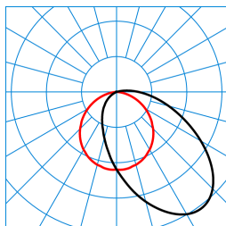
SanescaAct W2 5000 ETDD8/ET 840 03 ACTDSU (reading light) TX301999
