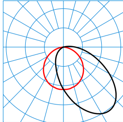
SanescaAct W2 5000 ETDD8/ET 840 03 ACTDWW (reading light) TX301996
