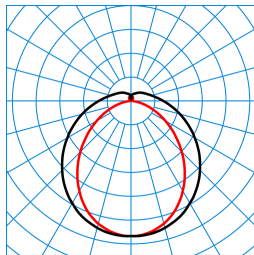
So-Tube G3 D/H3 DW 30-840 ETDD 05 TX773606
