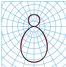
SFlow H2-L MRWD LED6400-830 ET 03 TX770320
