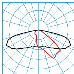
LIQ 50N-AB2L-LR/135/165/200-740 2G1 ET (CLO initial value) TX776370
