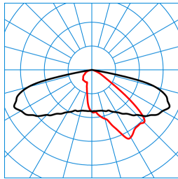
LIQ 50N-AB2L-LRA/1800-730 2G1 ETDD (CLO end value) TX778344
