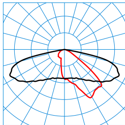
LIQ 50N-AB2L-LRA/1800-730 2G1 ETDD (CLO initial value) TX778350
