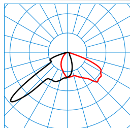
LIQ 70N-FL1L/9100-722 10G1 ET (CLO end value) TX778762
