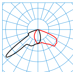
LIQ 70N-FL1L/9100-722 10G1 ET (CLO initial value) TX778767
