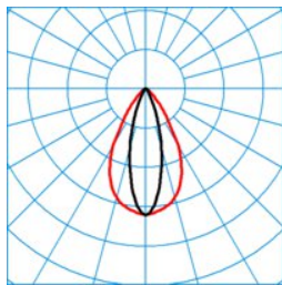
ELINE HE LEN60-160 ML 865 L225 2 20
