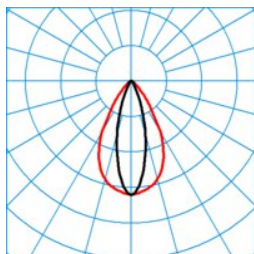
ELINE HE LEN60-160 ML 865 L225 4 20
