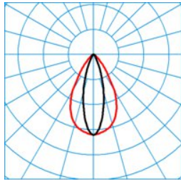
ELINE HE LEN60-160 ML 865 L225 0 20
