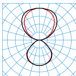
Luceos D/H2-L CDP 8400-840 ETDD 01 (Pendant ZS/ZST+EB3) TX547700
