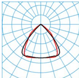
ELINE LW2240-110 ML 840 L150 4 50
