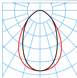
ArimoFit M46 DW19 IP 42-840 ET TX428856
