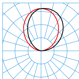
Sanesca W2 LED2600-830 03 (room light) TX046351
