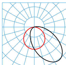
Sanesca W2 LED2600-830 03 (reading light) TX046350
