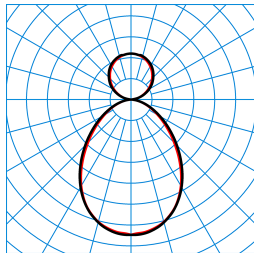
SFlow H2-L MRWD LED6400-840 ETDD 03 TX721249
