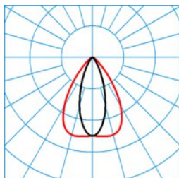
ELINE HE LVN60-160 ML 840 L225 4 20 ■ C0 - C180
