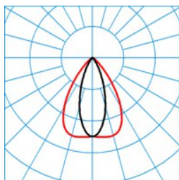
ELINE HE LVN60-160 ML 840 L225 2 20 ■ C0 - C180
