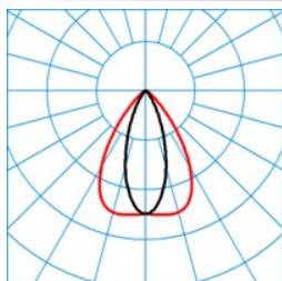
ELINE HE LVN60-160 ML 840 L225 0 20 ■ C0 - C180
