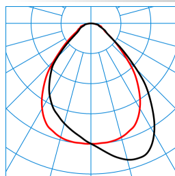
ArimoFit M46 P-WW 42-830 ET TX769016
