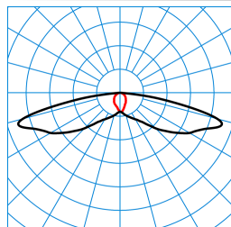
LIQ 50N-SB3L-LR/1350-722 2G1 ET (CLO end value) TX779596
