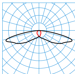
LIQ 50N-SB3L-LR/1350-722 2G1 ET (CLO initial value) TX779603
