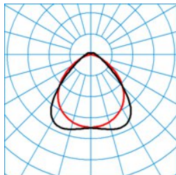
ELINE PW35-110 ML 865 L150 0 50
