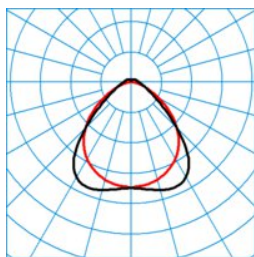
ELINE PW35-110 ML 865 L150 2 50
