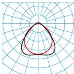
ELINE PW35-110 ML 865 L150 4 50
