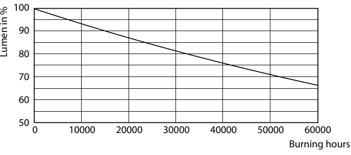
Lumen Maintenance Diagram - TForce LED HPL ND 38-28W E27 830
