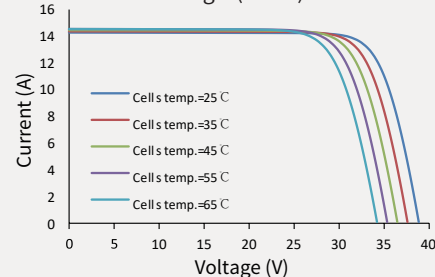
Current-Voltage (440W)
