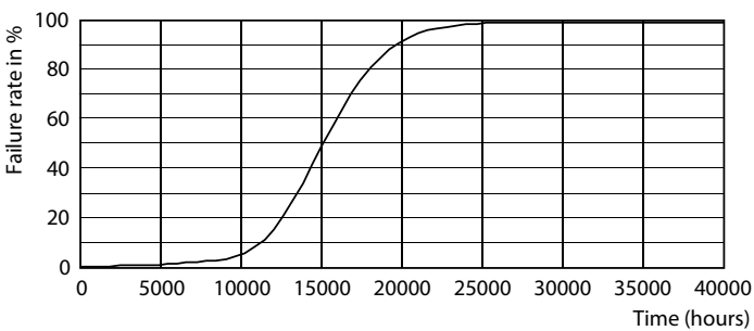
Life Expectancy Diagram - TForce Core HB MV ND 30W E27 840 G3
