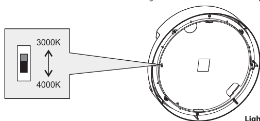
Light unit
