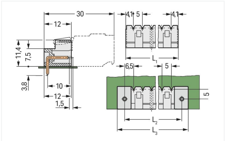
Dimensions in mm L1 = (pole no. – 1) x pin spacing + 8.2 mm L2 = L1 + 5 mm L3 = L2 + 7.4 mm
