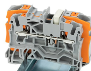
Step-down jumper (2006-499) commons 6/4 mm² (10/12 AWG) terminal blocks (2206/2204 Series) with 4/2.5/1.5 mm² (AWG 12/14/16) terminal blocks (2204/2202/2201 Series).
