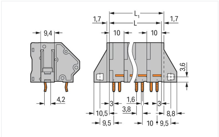
Dimensions in mm L = (\text{pole no.} - 1) \times \text{pin spacing} + 10 \text{ mm} L1 = L + 1.7 \text{ mm} \hat{=} version without mounting flange
