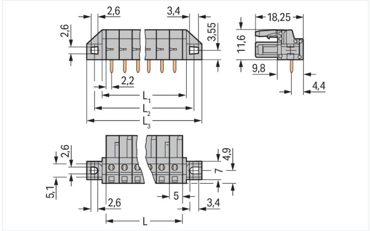
Dimensions in mm L = pole no. x pin spacing L1 = L + 3 mm L2 = L + 8.8 mm L3 = L + 14.8 mm 2- to 3-pole female connectors – one latch only
