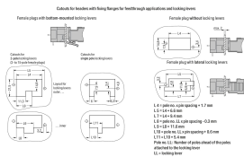
Cutouts for male headers with feed-through flanges and locking levers
