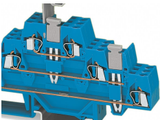
A vertical jumper commons the upper and lower decks, creating a 6-conductor feed-through terminal block in one housing. Two adjacent triple-deck terminal blocks may be commoned together on the same deck using a push-in adjacent jumper.
