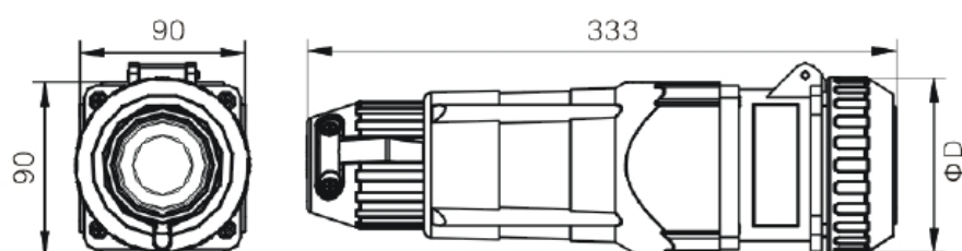
COUPLER SOCKET (all dimension in mm)
