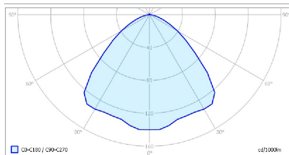
With external reflector
