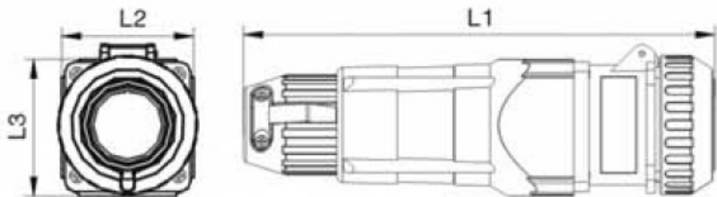
COUPLER SOCKET (all dimension in mm)
