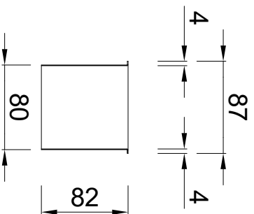
Doorsnede, 82mm
