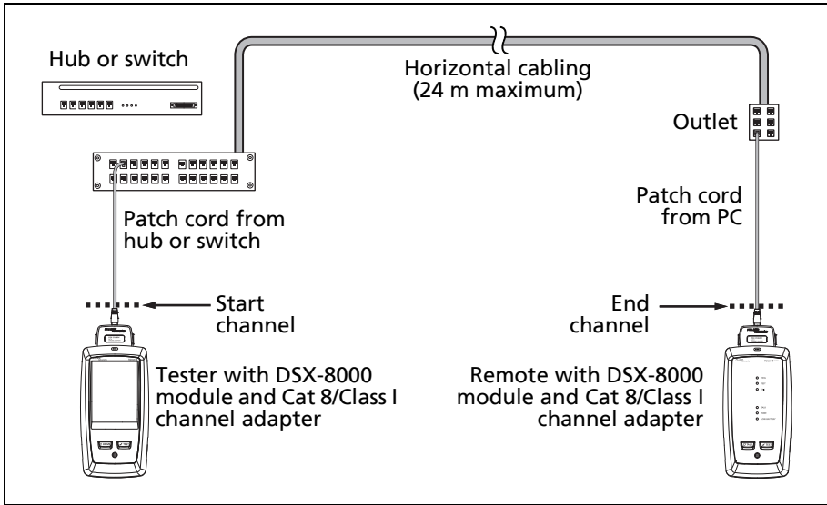
Figure 4. Channel Connections for Cat 8/Class I Links
