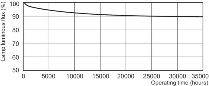
Lumen Maintenance Diagram - MASTER TL5 HE 35W/865 SLV/40
